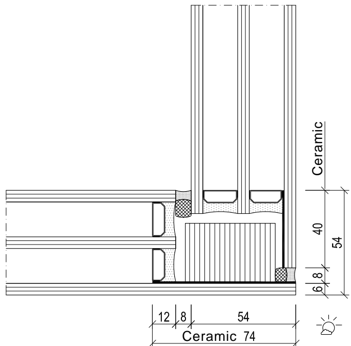
Fixed corner glazing with ceramic coating
